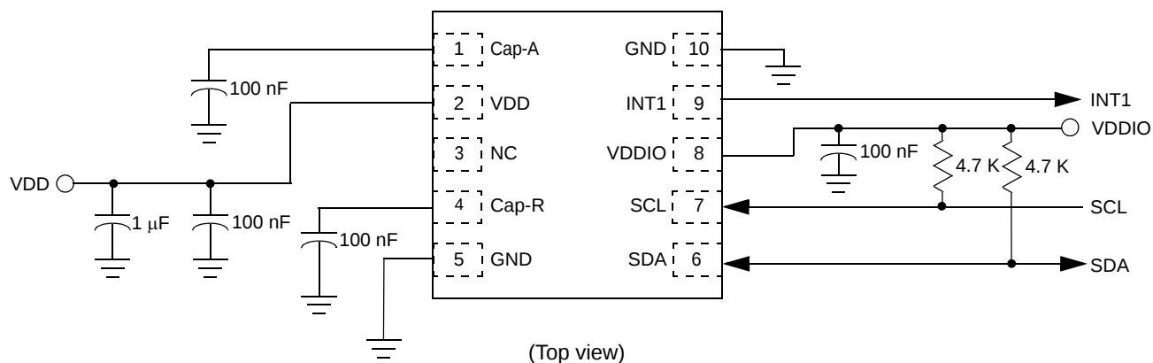
Figure 4. Electrical connection
